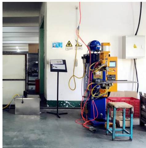
凸焊机 Projection welding machine
