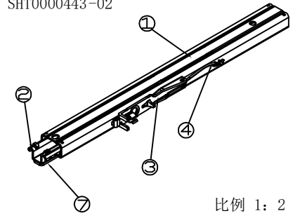
右滑轨 SHT0000443-02
