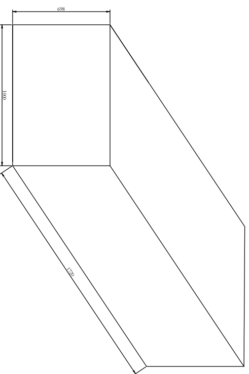
围板：外尺寸 1720x1000x698
